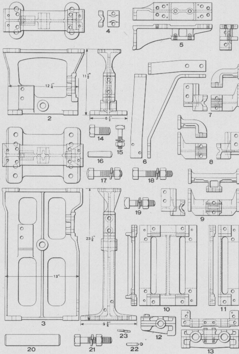
STANDS, FRONT AND BOTTOM RAILS, ETC., FOR DWARF INTERLOCKING MACHINE
